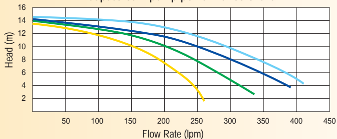
Supastream pump performance chart
